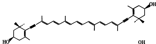
(3 R ,3' R )-7,8,7',8'-Tetrahydro- \beta , \beta -carotene-3,3'-diol
