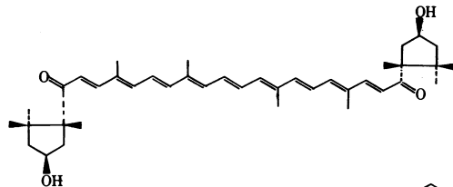
(3 S ,5 R ,3' S ,5' R )-3,3'-Dihydroxy- \kappa,\kappa -carotene-6,6'-dione
