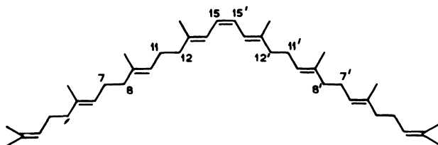
Natural phytoene = 15- cis -7,8,11,12,7',8',11',12'-octahydro- \psi,\psi -carotene
