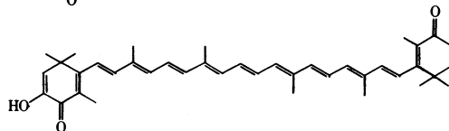
3-Hydroxy-2,3-didehydro- \beta,\beta -carotene-4,4'-dione
