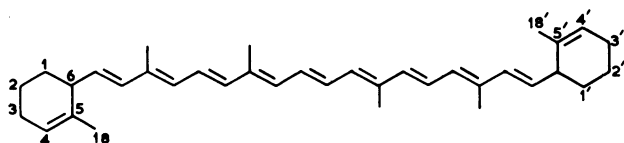
16.17,16',17'-Tetranor- \epsilon,\epsilon -carotene
