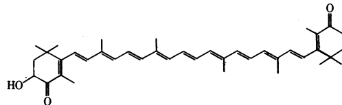
3-Hydroxy- \beta,\beta -carotene-4,4'-dione
