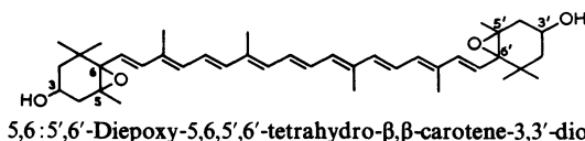
5,6:5',6'-Diepoxy-5,6,5',6'-tetrahydro- \beta,\beta -carotene-3,3'-diol
