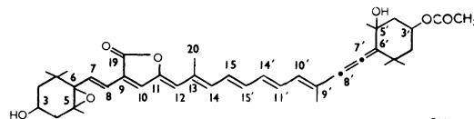
3'-Acetoxy-5,6-epoxy-3,5'-dihydroxy- 6',7'-didehydro-5,6,5',6'-tetrahydro- 12',13',20'-trinor- \beta,\beta -caroten- 19,11-olide
