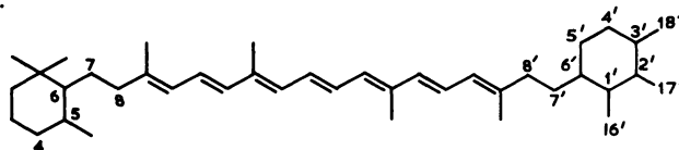
5,6,7,8,1',2',3',4',5',6',7',8'-Dodecahydro- \beta,\chi -carotene
