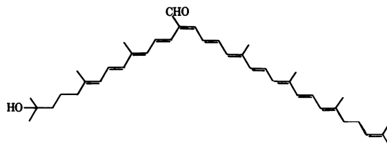
13- cis -1-Hydroxy-1,2-dihydro- \psi,\psi -caroten-20-al
