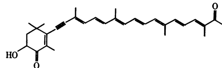
3-Hydroxy-7,8-didehydro-7',8'-dihydro-7'-apo- \beta -carotene-4,8'-dione or 3-hydroxy-8'-methyl-7,8-didehydro-8'-apo- \beta -carotene-4,8'-dione
