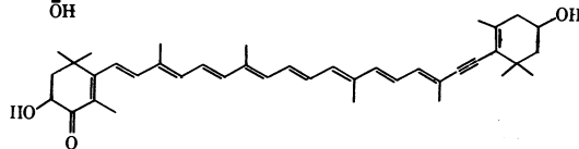
3,3'-Dihydroxy-7',8'-didehydro- \beta,\beta -caroten-4-one
