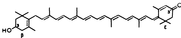
3-Hydroxy-6',7'-retro- \beta,\epsilon -caroten-3'-one
