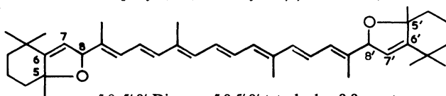
5,8:5',8'-Diepoxy-5,8,5',8'-tetrahydro- \beta,\beta -carotene
