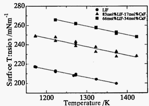
Fig. 3: Temperature dependence of surface tension of molten LiF-CaF 2 .
