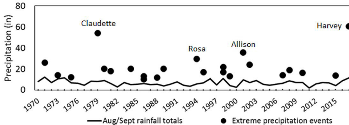
Figure 3. Texas rainfall during August-September (black line, averaged across weather stations, values from noaa.gov/cag, retrieved October 2017) compared to local records of highest rainfall during extreme precipitation events (here, defined as local rainfall above >10") associated with hurricanes (black circles, data from National Hurricane Center).
