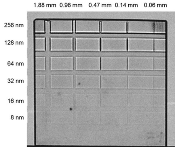
Figure 3: Striae reference plate with different wavefront steps achieved with coatings of different thickness and with gaps of different width.
