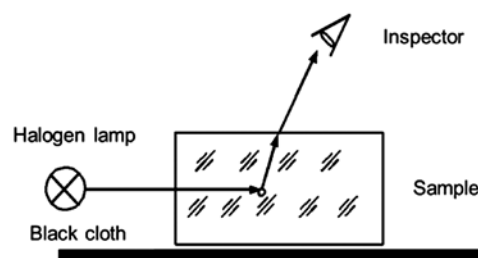
Figure 4: Inspection setup for bubbles and inclusions.
