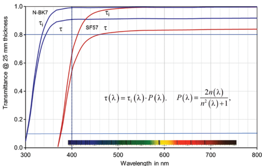
Figure 2: Transmittance ( \tau ) and internal transmittance ( \tau_i ) curves for two optical glasses, a low-refractive index glass N-BK7, and a high-refractive index glass SF57. P , Reflection factor; n , refractive index. The 80% and 10% lines are highlighted. The spectrum indicates the visible light range.
