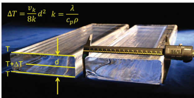
Figure 7: Thermal gradients depend on thickness square in the model of infinite plates. For low-temperature conducting materials such as glass (low k -value), special care has to be taken to keep them lowest possible while still achieving reasonable tempering periods.
