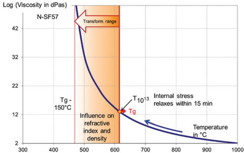
Figure 6: The cooling rate while crossing the transformation range determines essential properties of optical glass such as density and as consequence refractive index. Thermal gradients in the glass volume lead to spatial variation in refractive index and, thus, inhomogeneity. They also cause permanent residual stress at room temperature.
