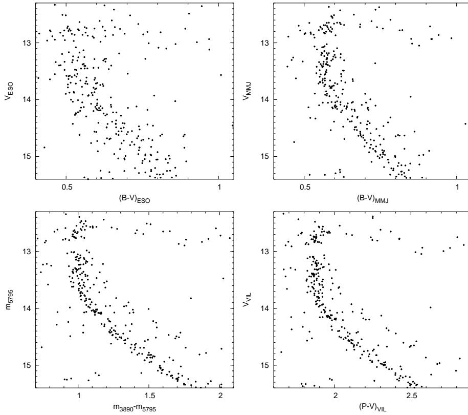
Fig. 4. The CMD diagram of M67 near the MS turnoff for stars in common to Vilnius, BATC, ESO and MMJ datasets. The sharpness of gaps in the MS at V \approx 13.0 and 14.2 mag and the sequences of subgiants and binaries can be used as the indicators of photometric accuracy.
