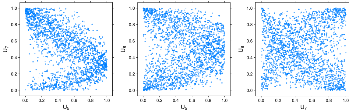
Figure 5: Scatterplots of pseudo observation ranks for pairs (left) f\text{Conc1}(U_5) and f\text{M3Long}(U_7) , (middle) f\text{Conc1}(U_5) and f\text{M3Trans}(U_8) and (right) f\text{M3Long}(U_7) and f\text{M3Trans}(U_8) from the MAGIC data set ( n = 2\,000 ).
