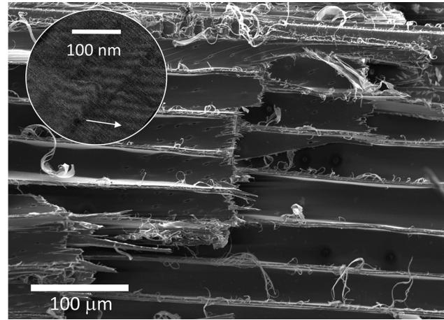
Figure 3: SEM image of the fracture surface of a Sitka spruce ( Picea sitchensis ) earlywood sample broken under tensile stress along the grain from left to right, showing (centre of image) a transverse crack across four cells associated with diagonal splits in pit fields with relatively high microfibril angle. The transverse crack is deflected into the longitudinal plane to the right and left, where the shear fracture in the longitudinal cell walls is ragged, with curled fibres consistent with the residues of bridging. The longitudinal fractures in this sample continued far beyond the right and left edges of the image and the ratio of the longitudinal to transverse fracture plane area was approximately 40–1. Inset: AFM image of the same sample at higher magnification showing a stepped fracture surface, with transverse cracks running across sheets of macrofibrils about 20 nm in thickness, and deflected into the longitudinal plane between these sheets. The arrow indicated the longitudinal direction of the macrofibrils.
