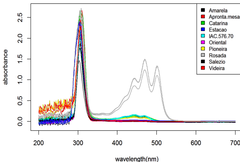
Figure 1: Typical UV-Vis spectrophotometric profiles ( \lambda = 200\text{-}700 nm, acetone: petroleum ether - v/v) of root parenchymal tissues of ten cassava genotypes cultivated in southern Brazil.
