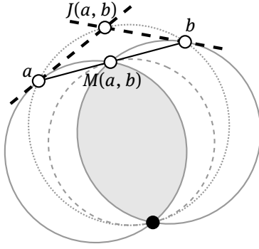
Figure 2: Computing the meet and join of the points a and b in the 2D (Euclidean) inner product sponge. The line segment between a and b is the convex hull of those two points. Each point has an associated circle enclosing all of its lower bounds (the dark dot represents the origin). The thick, dashed lines show the boundaries of the half-spaces of upper bounds for a and b . The shaded area below the meet is the intersection of the lower bounds of a and b , and is a subset of the set of lower bounds of the meet, consistent with part preservation.
