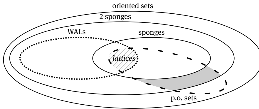
Figure 1: An Euler diagram of the oriented and ordered structures discussed in the text. The shaded area is empty, but all other areas are not. The set of all lattices is the (hatched) intersection of WALs and p.o. sets.
