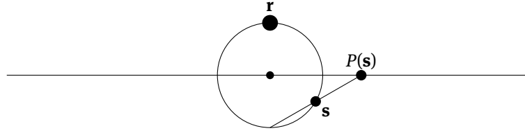
Figure 3: Stereographic projection projects points on the unit circle (hypersphere) onto a line (hyperplane) through the origin (smallest black dot) along lines emanating from the antipode of the reference point \mathbf{r} .
