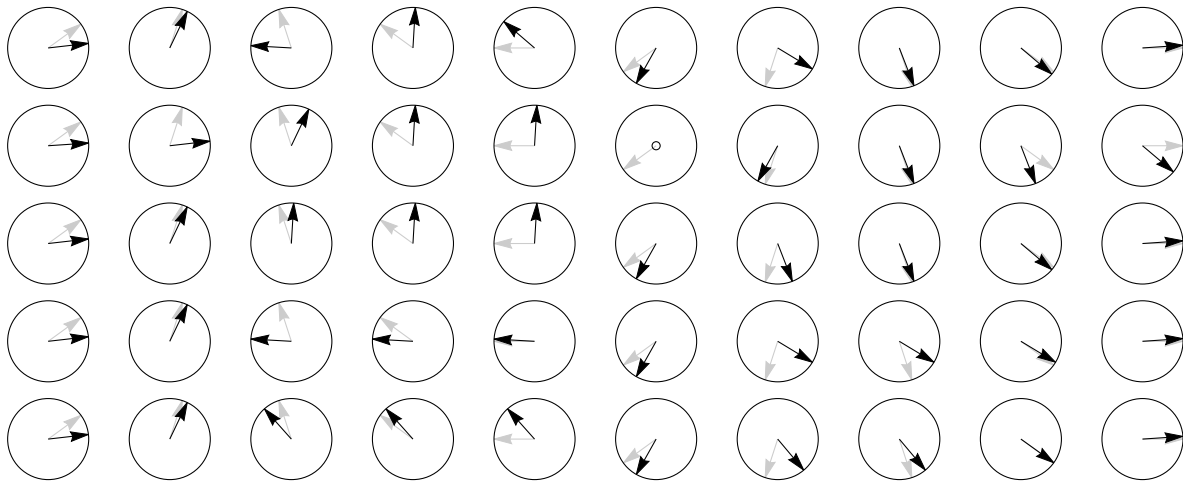
Figure 5: From top to bottom (black arrows): The original 1D angle-valued signal (the grey arrows plus noise), the result of a structural pseudo-erosion, the result of a structural “opening”, the result of the corresponding “closing”, and the average of the two. The empty circle and lack of arrow in one of the circles on the second row indicate that for that position no angle could be given as the meet, resulting in a special “bottom” value instead. The operators were computed using a flat structuring element consisting of three adjacent positions, using periodic boundary conditions. Source code available at http://bit.ly/1Rz8SVp .
