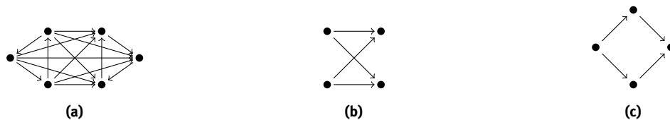
Figure 7: (a) An orientation of six elements that is a WAL, but not a sponge (arrows point in the direction of larger values). There are two cycles, with every element in the right cycle being an upper bound of every element in the left cycle. (b) An orientation that is not a 2-sponge. (c) A sponge that violates weak transitivity.
