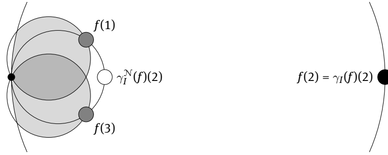
Figure 6: Illustration of the difference between \gamma_I as defined in Eq. (3) and \gamma_I^N as defined in Eq. (4), using the 2D inner product sponge. The set I is the same set used in the proof of Theorem 8, with the structuring element consisting of just two adjacent positions. The grey area associated with f(1) is the set of weights that make the (translated) structuring element \{1, 2\} a lower bound of f , the grey area associated with f(3) shows the same for the structuring element \{2, 3\} . Circles indicate boundaries of sets of lower bounds of points. The origin is depicted by a small black dot.
