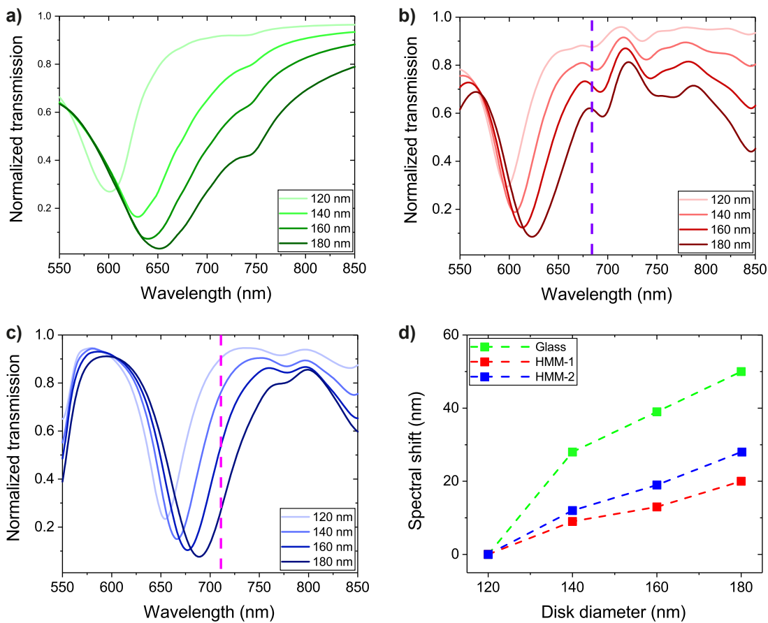
Figure 2: Evolution of the plasmon resonance with varying diameters of NDs on (a) glass (b) HMM-1, (c) HMM-2, and (d) spectral shift of the resonance, calculated by FDTD simulations. FDTD, finite-difference time-domain; HMM, hyperbolic metamaterial; ND, nanodisk.
