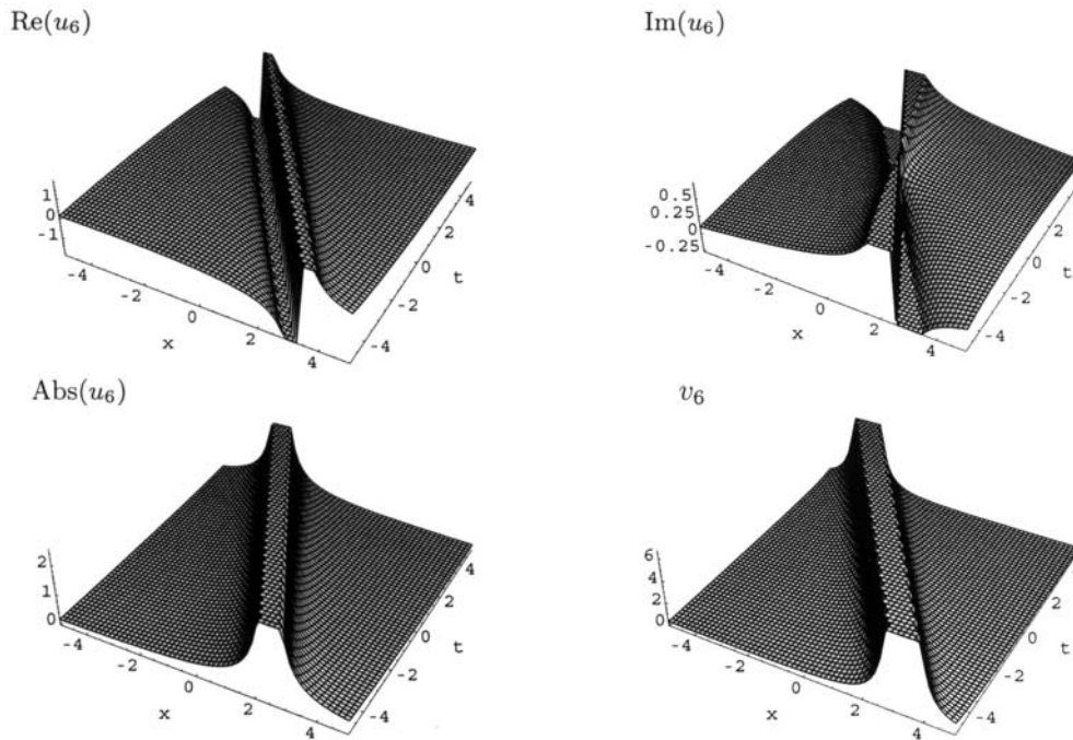
Fig. 7. The rational solutions u_6 and v_6 , where p = 0.3, a_1 = 1 .
