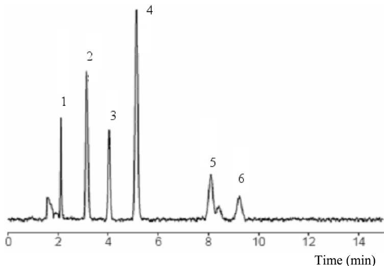
Fig. 2. RP-HPLC isocratic separation: standard solution analysis, detection at 254 nm. Mobil phase: water/acetonitrile (65:35, v/v, adjusted to pH 2.3 by ortho -phosphoric acid), flow rate 1.0 ml/min. 1, Caffeic acid; 2, myricetin; 3, morin; 4, quercetin; 5, apigenin; 6, kaempferol.
