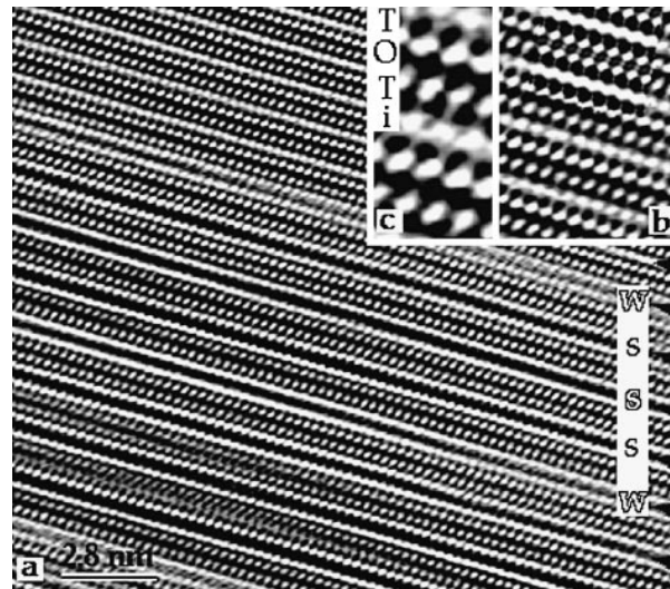
FIGURE 6. (a) Rotationally filtered Scherzer defocus [010] image of partially altered chlorite ( bottom ) and associated 1.0 nm phase. Arrows indicate brucite-like interlayers with variable S (strong) vs. W (weak) contrast. To our knowledge, [010] zone axis atomic-resolution images of layer silicates have not been previously published. Consequently, the area in (b) is enlarged (with superimposed image simulation) and in (c) is labeled to show the correspondence between tetrahedral cations (spots), the octahedral sheet (spotty stripes) and the interlayer. Simulations and details for chlorite are shown elsewhere.
