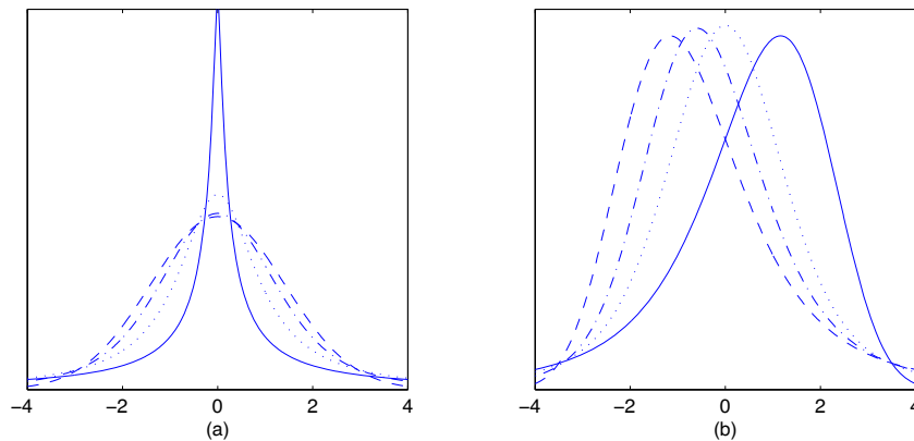
Figure 1: Density plot of \alpha -stable distribution with location parameter \mu = 0 and \gamma = 1 . (a) \beta = 0 . Solid line: \alpha = 0.5 . Dotted line: \alpha = 1 . Dash-dotted line: \alpha = 1.5 . Dashed line: \alpha = 2 . (b) \alpha = 1.5 . Solid line: \beta = -1 . Dotted line: \beta = 0 . Dash-dotted line: \beta = 0.5 . Dashed line: \beta = 1 .
