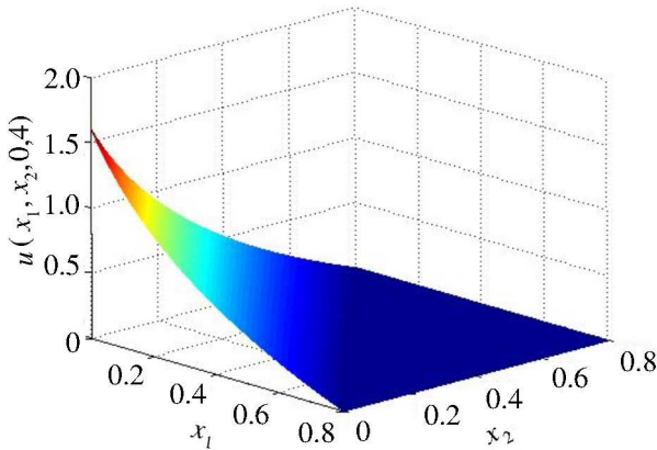
Fig. 4.5. Exact solution of problem (4.3) for t = 0.4, l_1 = 0.8, l_2 = 0.8, T = 0.4 and \lambda = 2
