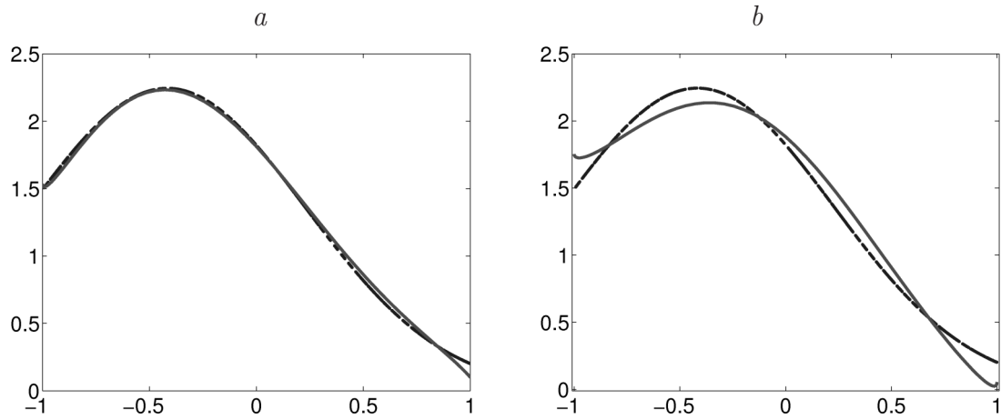
Fig 4.5. Reconstruction of the boundary function u^+ on the parabolic cut: exact data, k^* = 3000 (a); 5% noise, k^* = 145 (b)
