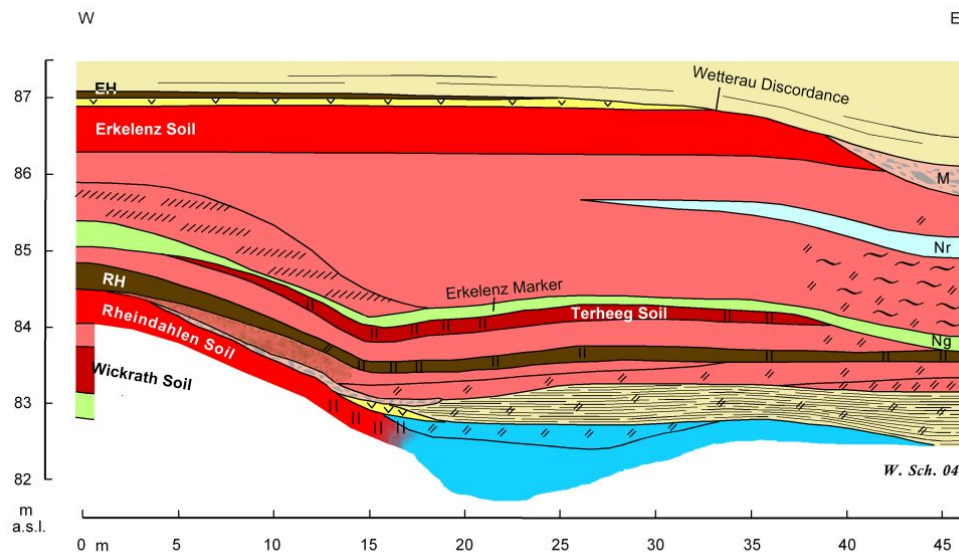
Figure 4. Section Erkelenz 25 shows the Erft Solcomplex (OIS 7) in a depression. Between the Rheindahlen and the Erkelenz Soil the Terheeg Soil (Bw horizon) is visible at a length of 35 m at the border of a depression only. EH = Erkelenz Humus Zone, M = soil sediment, Ng = speckled gelic gleysol, Nr = grey gelic gleysol, RH = Rheindahlen Humus Zone. Legend see Figure 1.
