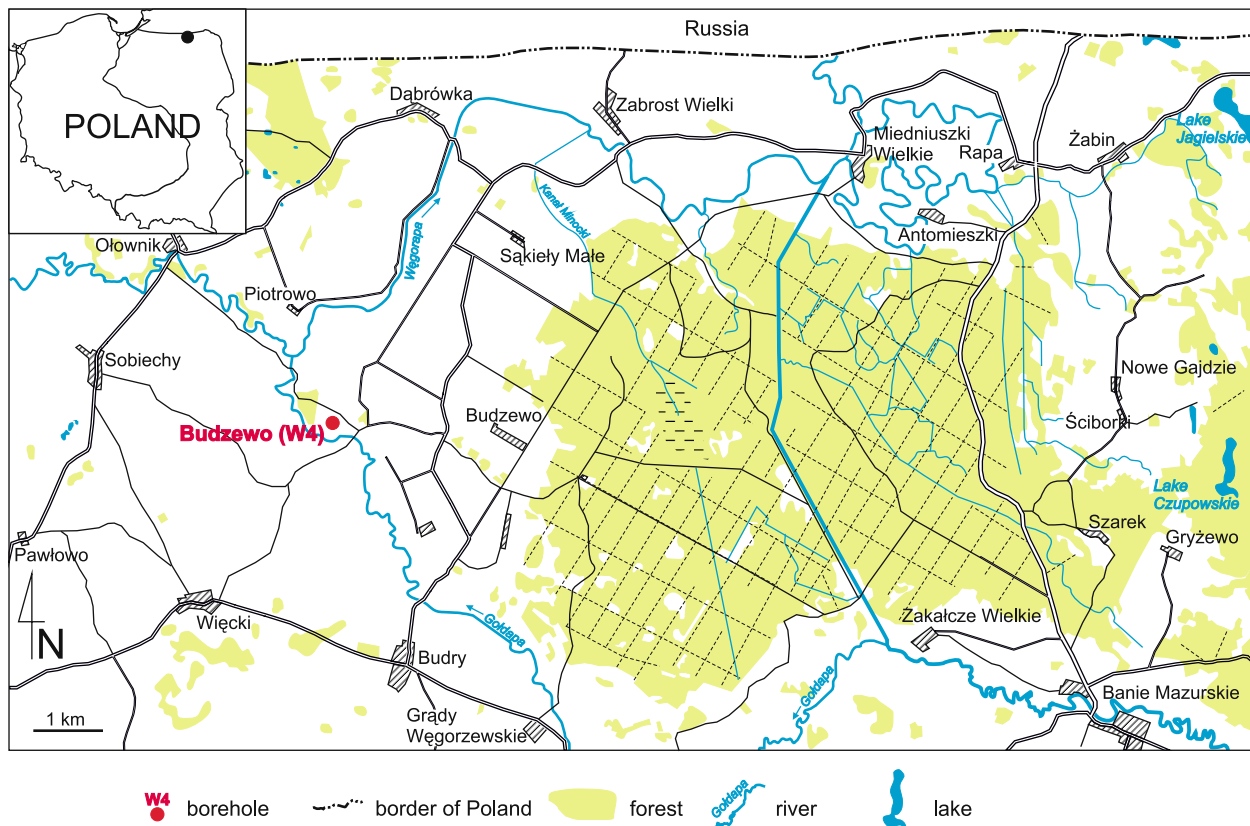
Fig. 1. Location of studied sediment sequence
