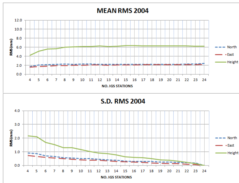
Fig. 4. Statistics obtained from varying number of IGS stations used in a mapping process for the 2004 campaign Top: Mean RMS values; Bottom: S.D. of RMS values.
