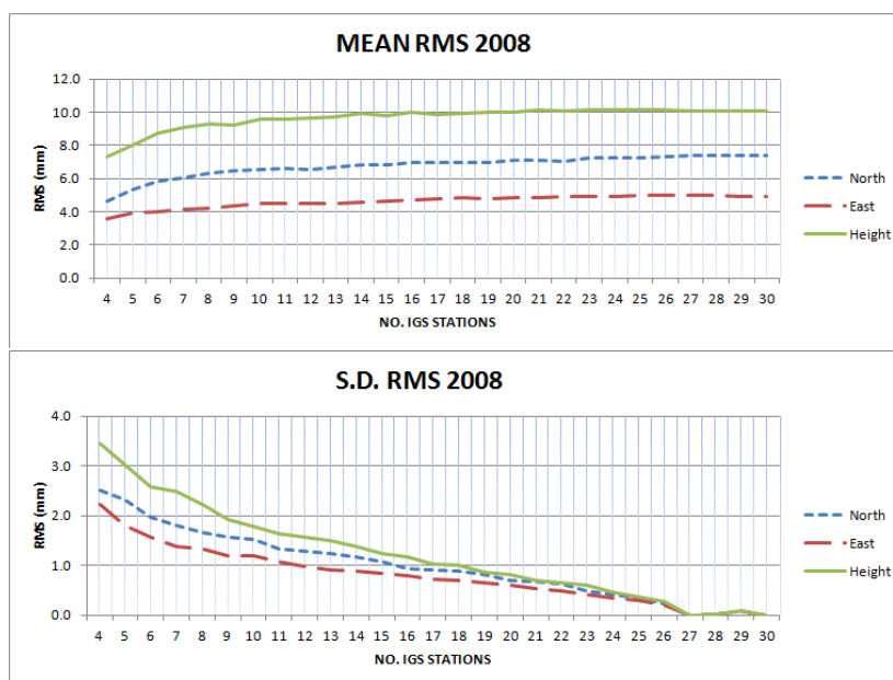
Fig. 5. Statistics obtained from varying number of IGS stations used in a mapping process for the 2008 campaign Top: Mean RMS values; Bottom: S.D. of RMS values.
