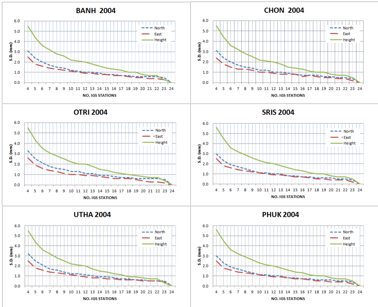
Fig. 6. Standard Deviation of final Thai coordinate solutions from the 2004 campaign.
