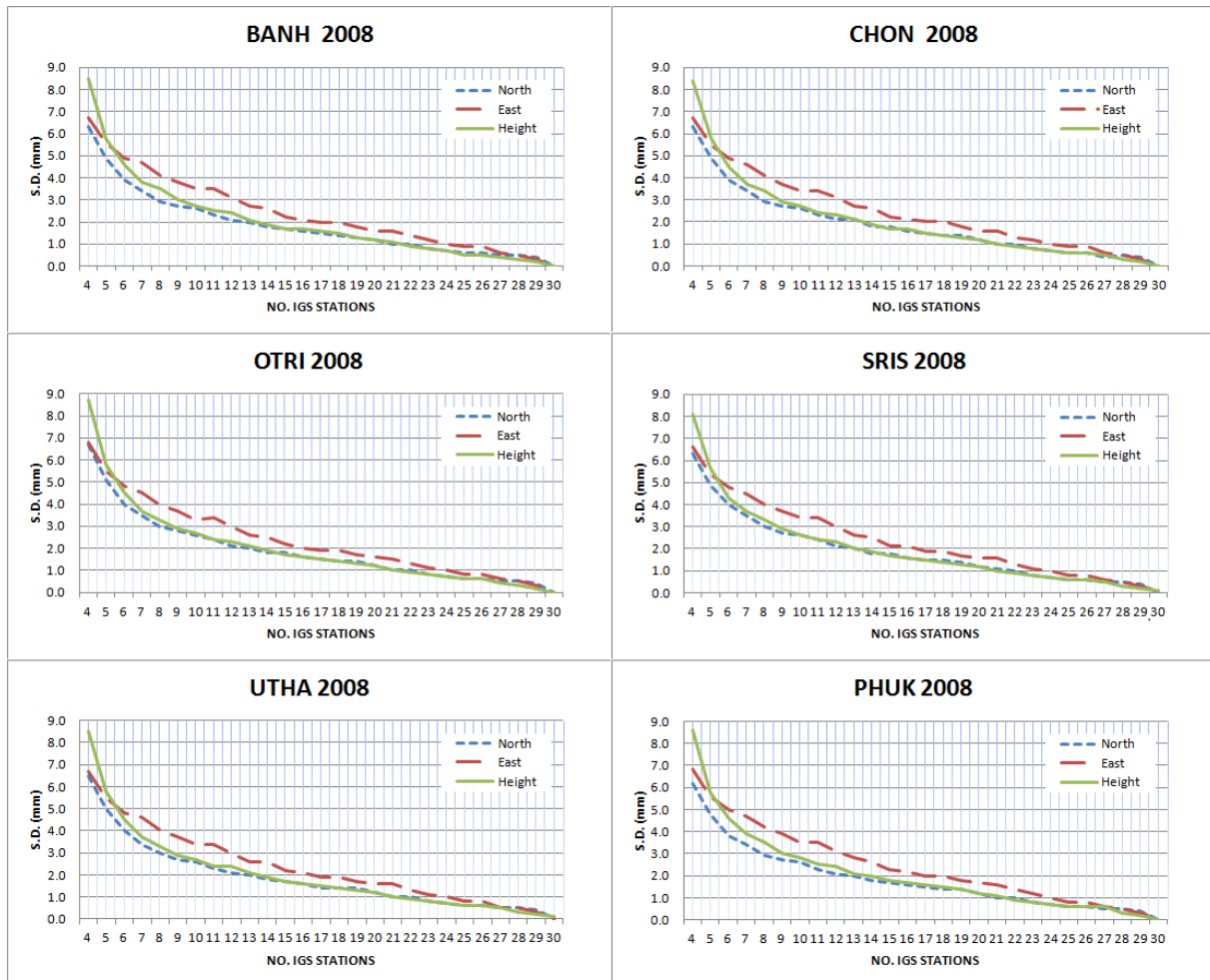
Fig. 7. Standard Deviation of final Thai coordinate solutions from the 2008 campaign.
