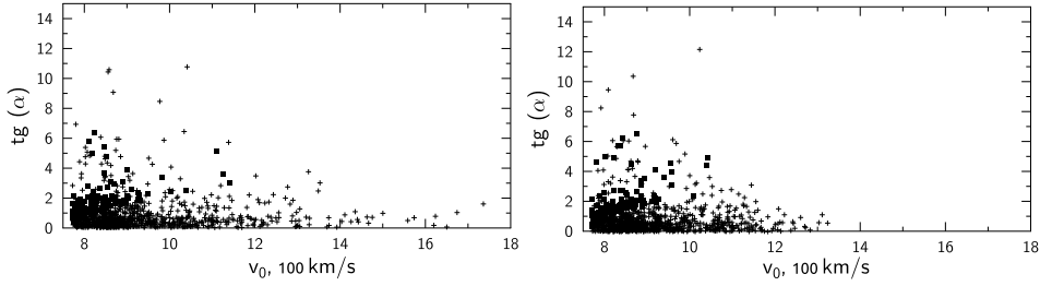
Fig. 1. The distribution of the angle \alpha between the initial velocity vector and the Galactic plane versus the initial velocity v_0 of the star, in the units of 100 \text{ km s}^{-1} , for simulations with the semimajor axis of a binary system equal to 282 R_\odot and the pericentric distances 10\,000 R_\odot (the left panel) and 15\,000 R_\odot (the right panel). The pluses and squares denote the hypervelocity and non-escaping stars, respectively.
