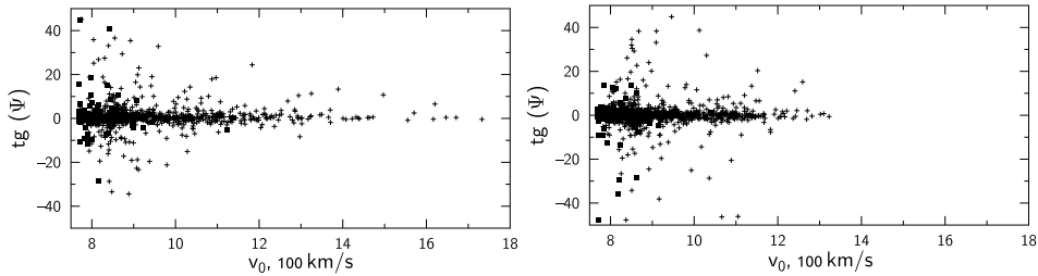
Fig. 2. The angle \psi between the initial velocity vector and the semimajor axis of the bar versus the initial velocity v_0 of the star, in the units of 100 \text{ km s}^{-1} , for simulations with the semimajor axis of a binary system equal to 282 R_\odot and the pericentric distances 10\,000 R_\odot (the left panel) and 15\,000 R_\odot (the right panel). The pluses and squares denote the hypervelocity and non-escaping stars, respectively.
