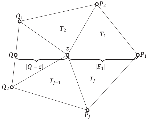
Figure 1. Geometry of a patch \omega_z^{(\ell)} \subseteq \mathbb{R}^2 for k = 1 in Section 3.10 to illustrate the convex coefficient \mu in z = \mu P_1 + (1 - \mu)Q for n = 2 .
