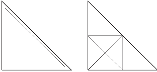
Figure 2. Reference triangle T (left) with reference edge marked, and bisec5(T) (right) in Section 4.1.
