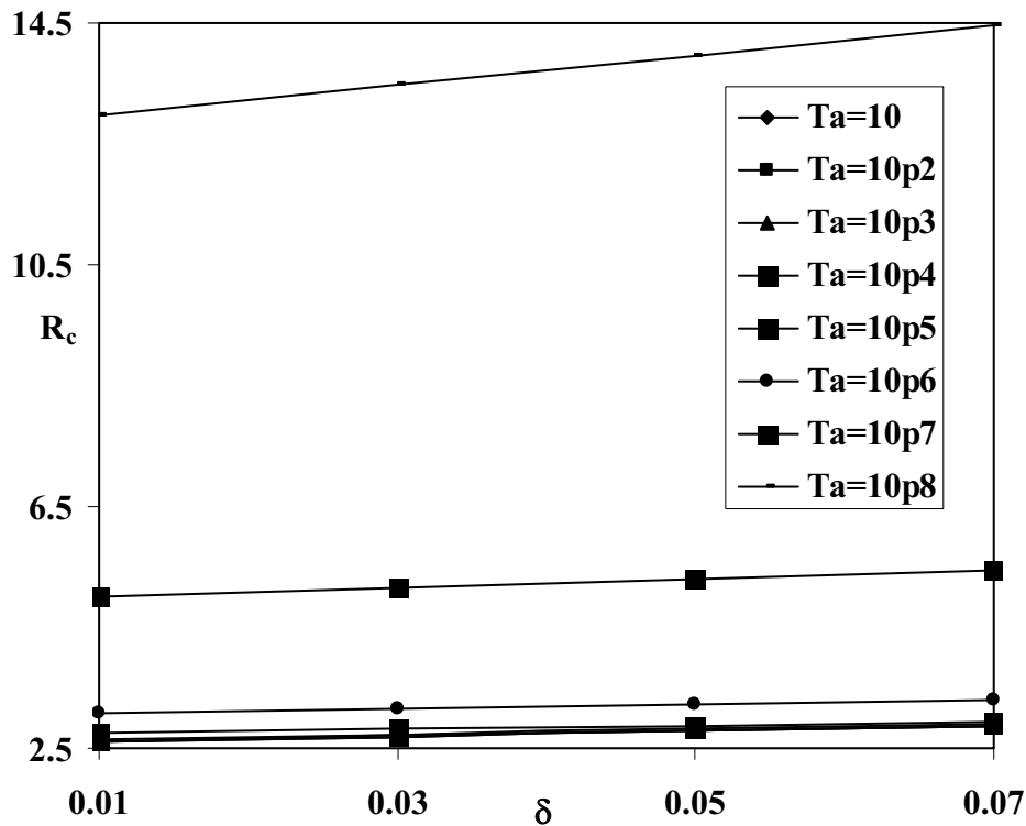
Fig.6. Variation of R_c versus \delta or different values of Ta .
