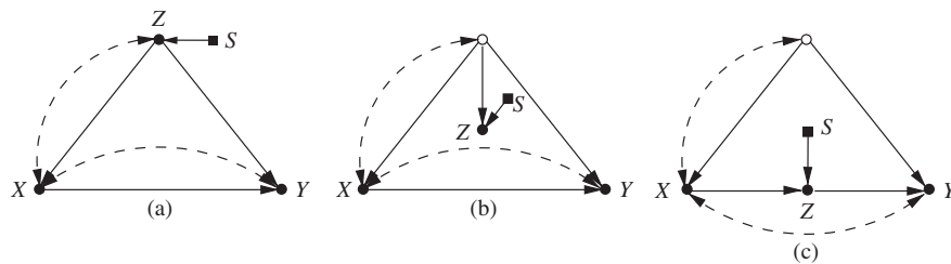
Figure 3 Selection diagrams depicting differences in populations. In (a), the two populations differ in age distributions. In (b), the populations differs in how reading skills ( Z ) depends on age (an unmeasured variable, represented by the hollow circle) and the age distributions are the same. In (c), the populations differ in how Z depends on X . Dashed arcs (e.g. X \dashrightarrow Y ) represent the presence of latent variables affecting both X and Y .
