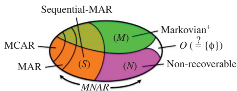
Figure 5 Recoverability of the joint distribution in MCAR, MAR, and MNAR. Joint distributions are recoverable in areas marked (S) and (M) and proven to be non-recoverable in area (N).
