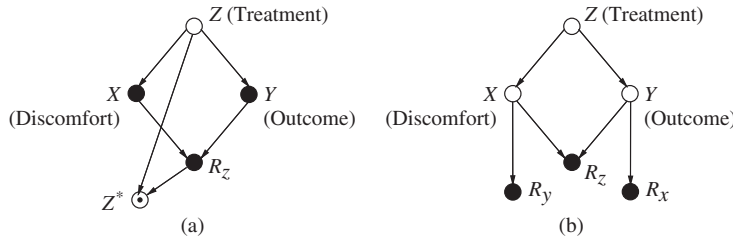
Figure 4 (a) Graph describing a MAR missingness process. X and Y are fully observed variables, Z is partially observed and Z^* is a proxy for Z . R_z is a binary variable that acts as a switch: Z^* = Z when R_z = 0 and Z^* = m when R_z = 1 . (b) Graph representing a MNAR process. (The proxies Z^* , X^* , and Y^* are not shown.)
