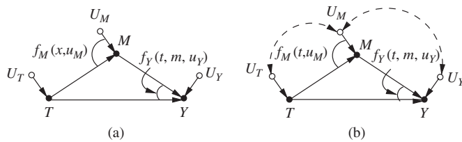
Figure 2 (a) The basic nonparametric mediation model, with no confounding. (b) A confounded mediation model in which dependence exists between U_M and (U_T, U_Y) .
