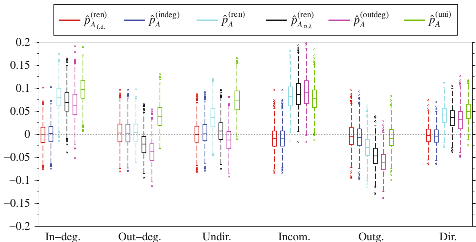
Fig. 5. Deviations of estimated p_A from the true population proportion in the power-law networks for \gamma = 3, E(D^{(un)}) = 4, E(D^{(in)} + D^{(out)}) = 12, p = 0.2, and n_s = 500. Each group of boxplots corresponds to \hat{p}_{A f.d.}^{(ren)}, \hat{p}_A^{(indeg)}, \hat{p}_A^{(ren)}, \hat{p}_{A \alpha,\lambda}^{(ren)}, \hat{p}_A^{(outdeg)}, and \hat{p}_A^{(uni)} , for one allocation of A.
