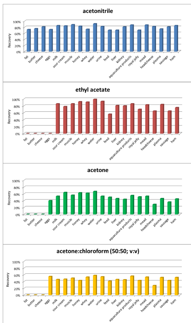
Fig. 3. Comparison of suitability of different extraction solvents for chloramphenicol
