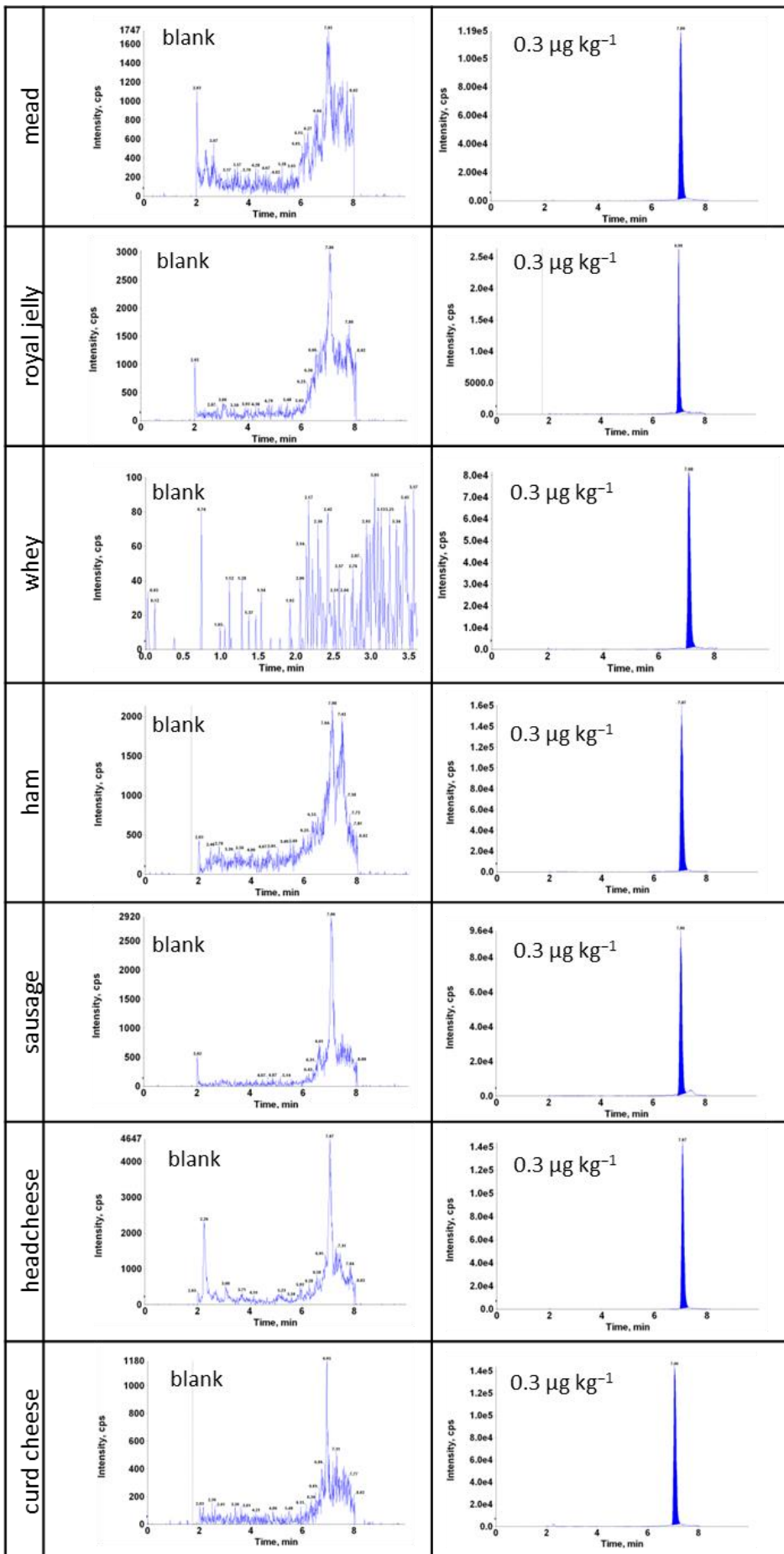
Fig. 2. Chromatograms of different matrices, blank and CAP spiked sample ( 0.3 \mu\text{g kg}^{-1} )
