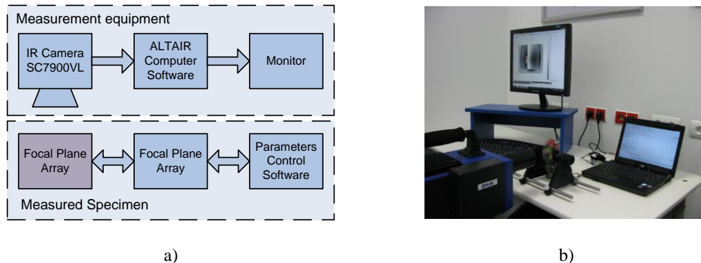
Fig. 6. Measurements stand for microbolometric array evaluation: block diagram (a) and real setup (b).
