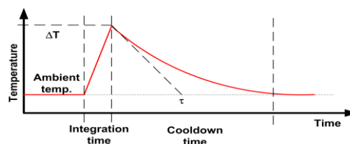
Fig. 10. Theoretical thermal behavior of the detector.
