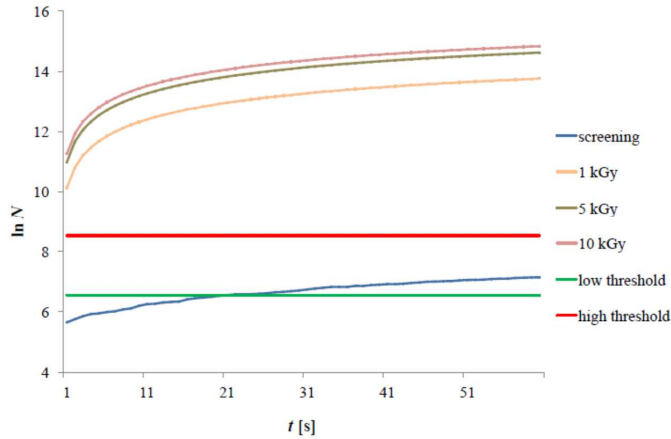
Fig. 3. The PSL measurements of paprika standard for an unirradiated sample (screening method) and samples treated with doses of 1 kGy, 5 kGy and 10 kGy (Co-60 as an irradiation source).
