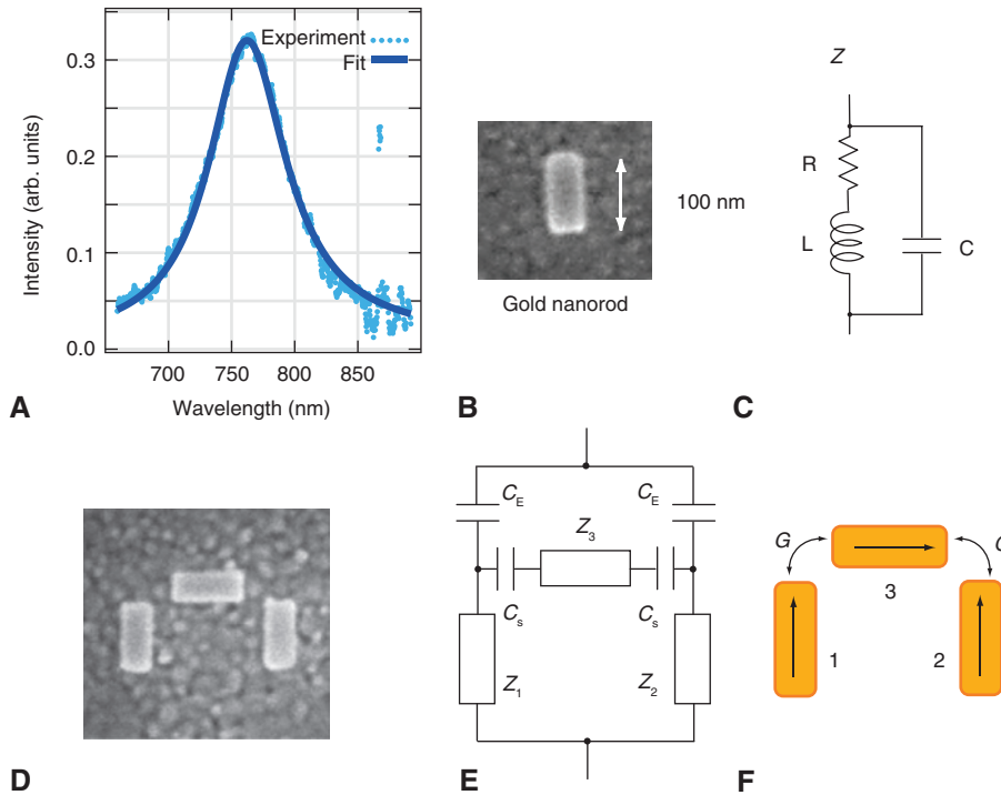
Figure 6: Plasmonics as electronics. (A) An example of the scattering spectrum from a single gold nanorod l=100 nm, w=40 nm, t=30 nm; (B) SEM image of the resist used to define a gold nanorod during lithography; (C) the equivalent circuit impedance of the rod – the spectrum is fit to I=A+B|Z|^2 where Z=(R+j\omega L)/(1-\omega^2 LC+j\omega RC) is the circuit impedance. The fit gives the lumped component values RC=3.99 \times 10^{-17} s and LC=1.64 \times 10^{-31} s 2 and the resonant frequency is f=1/2\pi\sqrt{LC}=393 THz; (D) a three-nanorod structure that mimics a Wheatstone bridge circuit [150, 151]; (E) the equivalent electrical circuit; (F) an alternative analysis using plasmon coupling theory [152] that gives plasmon excitation amplitude on nanorod 3 \tilde{a}_3=[Gp \cdot (E_1 - E_2)]/[(\delta\omega + i\Gamma/2)^2 - 2G^2] directly in terms of parameters associated with the optics of nanoparticles – the detuning \delta\omega from the single rod resonance of FWHM \Gamma , dipole moment p and interparticle coupling G . The LSP amplitude depends on the difference in the electric fields E_1 - E_2 of the light incident on the two parallel rods, 1 and 2.
