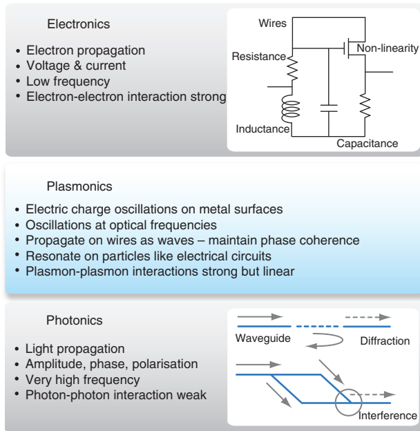
Figure 1: A comparison between electronic and photonic circuits. The field of plasmonics lies in between.
