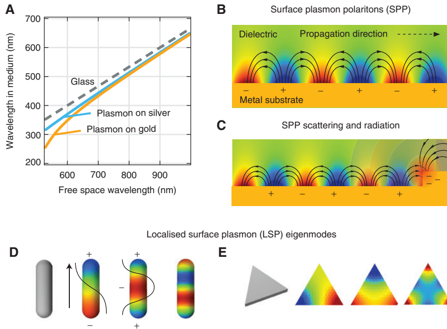
Figure 2: Plasmons propagating on surfaces: (A) The wavelength of an SPP is shorter than the free space wavelength of light or the wavelength within the dielectric, which prevents the plasmon from radiating; (B) the electric field associated with an SPP propagating over the surface of a thick metal film; (C) illustration of a plasmon scattering at a discontinuity with some energy converted to radiation in the dielectric; (D–E) examples of LSPs on different metal particles. These show the charge distributions (blue positive, red negative) of different resonant modes. The fundamental mode is a half wavelength with a strong dipole moment.
