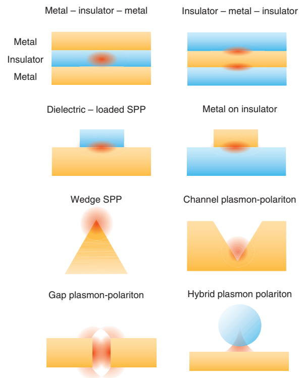
Figure 3: Cross sections of different types of plasmon waveguides (adapted from Ref. [18]).
