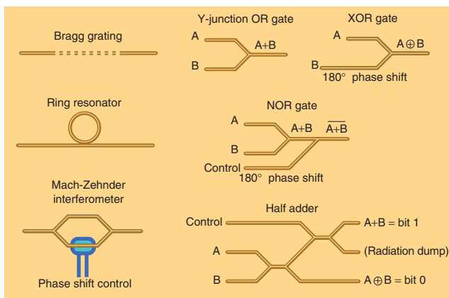
Figure 4: Plasmonic waveguide devices for performing optical processing. The logic circuits operate using phase shifts and interference.
