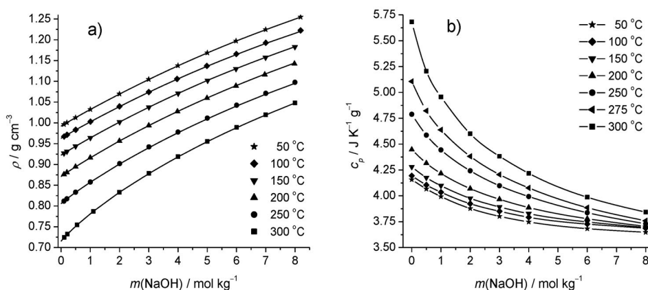
Fig. 2 (a) Densities [3] and (b) heat capacities [6] of NaOH(aq) up to 8 mol kg -1 at temperatures from (50 to 300) °C and a pressure of 10 MPa.
