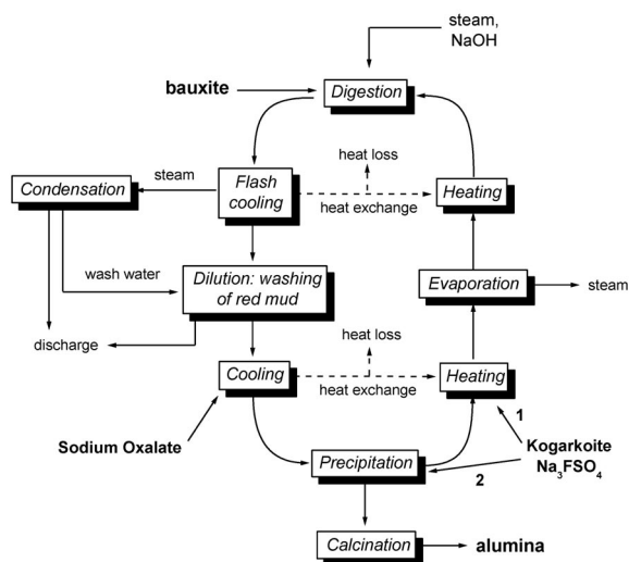
Fig. 6 Simulation of the accumulation of oxalate and fluoride in a Bayer process circuit [22]. The process stages in which liquors first become supersaturated with respect to sodium oxalate and kogarkoite, respectively, are indicated by arrows. Boxes indicate equilibrium calculations.
