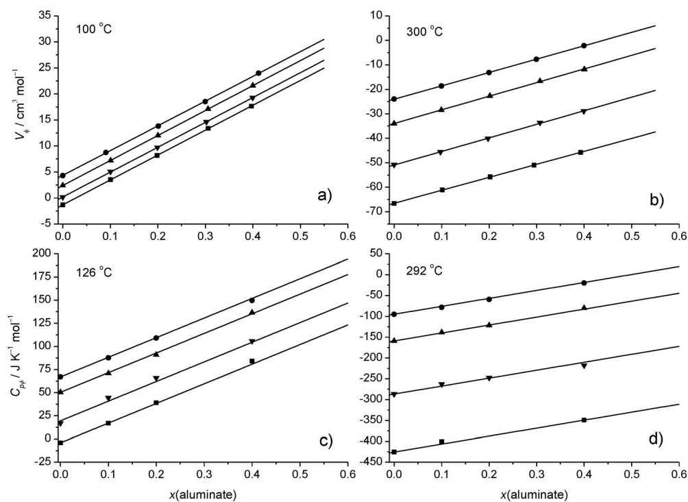
Fig. 3 Apparent molar volumes (a, b) and heat capacities (c, d) of aqueous NaOH + “NaAl(OH) 4 ” mixtures as a function of aluminate substitution at constant ionic strengths I/\text{mol kg}^{-1} of 1 (■), 2 (▼), 4 (▲) and 6 (●) at various temperatures and a pressure of 10 MPa.
