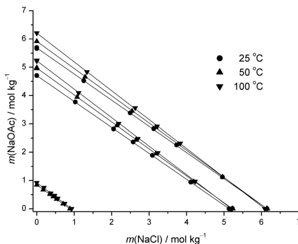
Fig. 4 Isopiestic molalities in the ternary NaOAc + NaCl + H 2 O system measured at (25 to 100) °C. Each series corresponds to a constant water activity; the lines indicate Zdanovskii’s rule.
