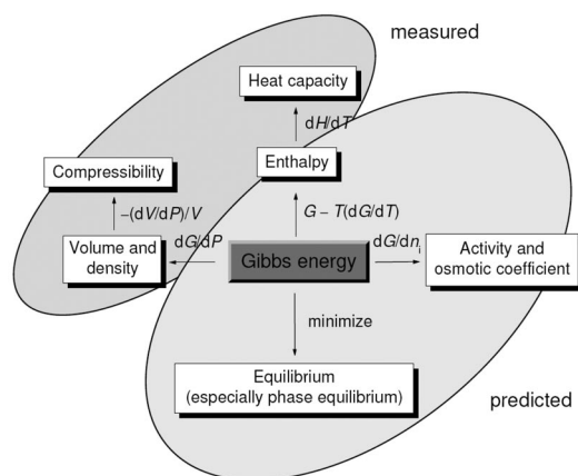
Fig. 1 Thermodynamic consistency indicated by thermodynamic relationships among measurable quantities. The shaded areas relate to the experimental and modeling strategy applied in this work.
