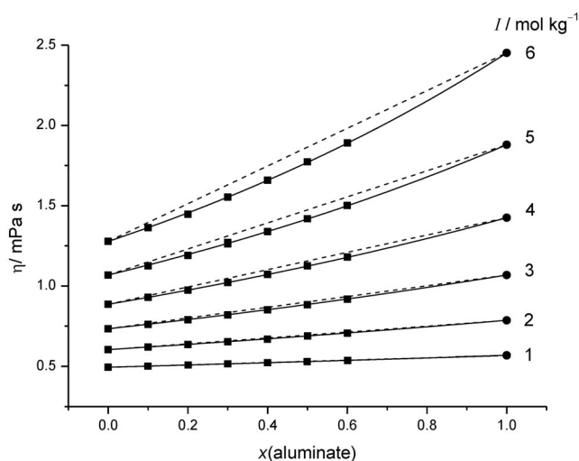
Fig. 5 Viscosities in the ternary \text{NaOH} + \text{NaAl}(\text{OH})_4 + \text{H}_2\text{O} system as a function of aluminate substitution at constant ionic strengths I at 70^\circ\text{C} (squares). Solid lines, Zdanovskii's rule; dashed lines, "Young's rule"; dots, extrapolated viscosities of hypothetical, pure " \text{NaAl}(\text{OH})_4(\text{aq}) ".
