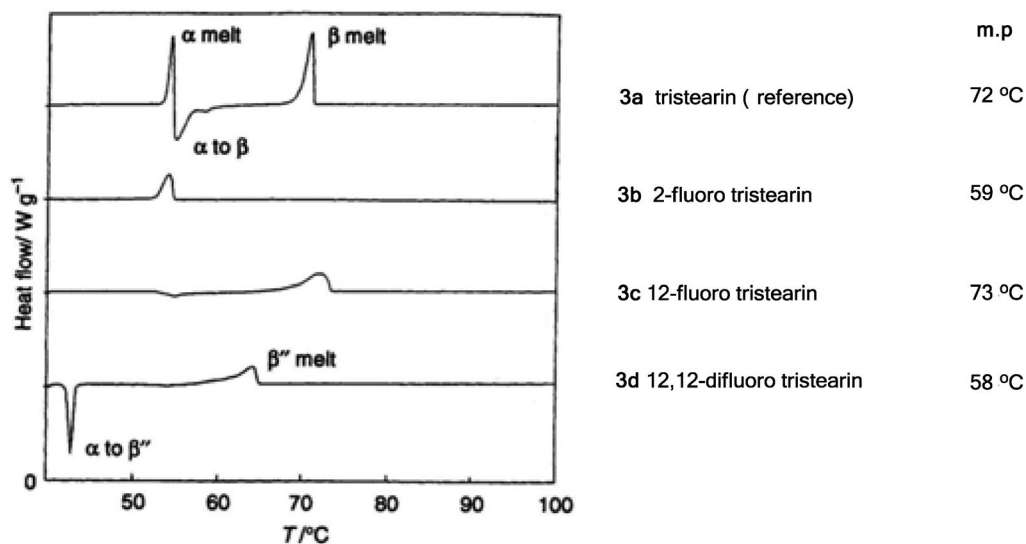
Fig. 10 DSC thermogram of tristearin 3a and fluorinated tristearins 3b–d [9].
