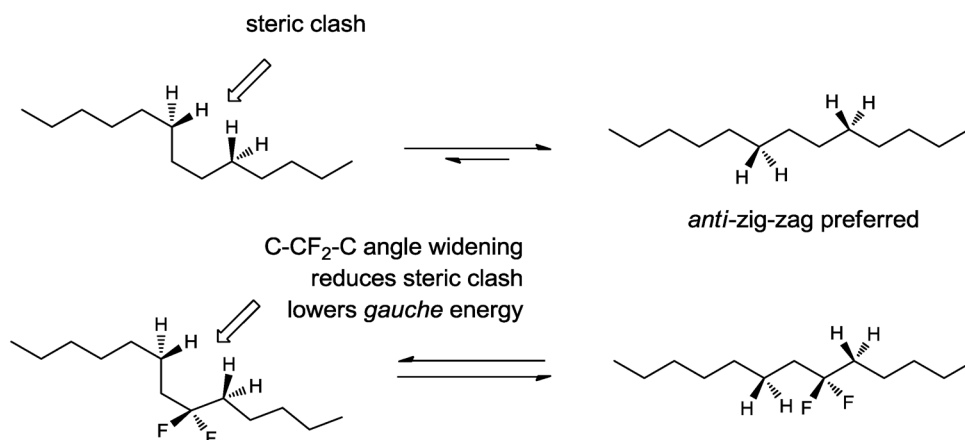
Fig. 11 CF 2 -functionalized aliphatic chain introduce increased conformational disorder.
