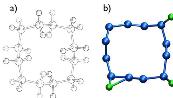
Fig. 12 (a) Dunitz and Shearer cyclododecane X-ray derived structure [24]. (b) Disordered 1,1-difluoro-cyclododecane structure [10].
