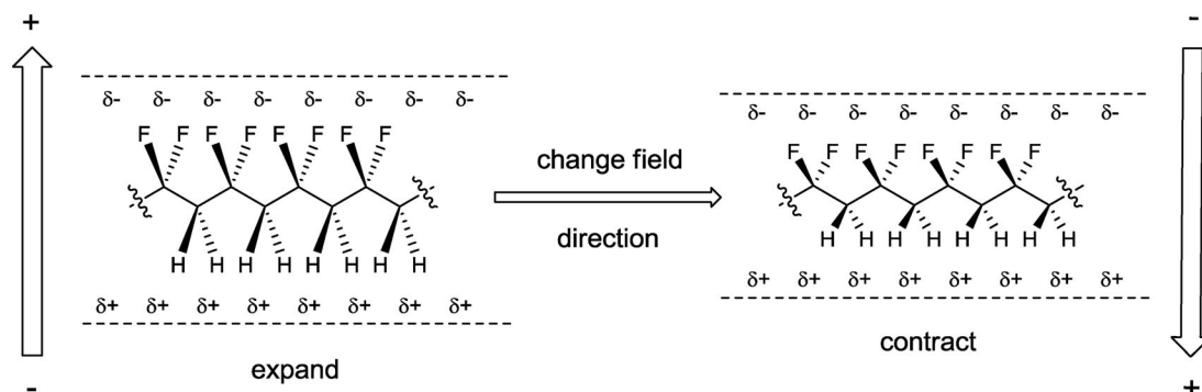
Fig. 5 The piezoelectric response of PVDF in an alternating electric field.
