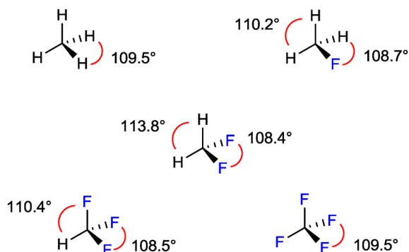
Fig. 3 Bond angles in methane and the fluoromethane series.
