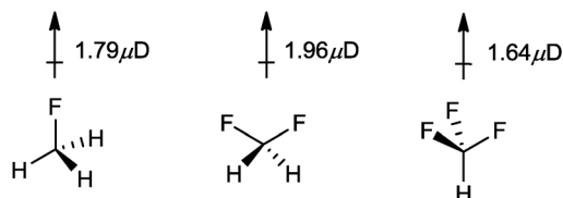
Fig. 4 Dipole moments of fluorinated methanes [14].
