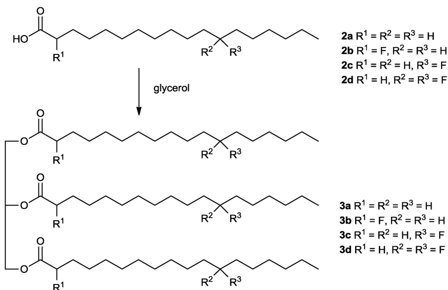
Fig. 9 Preparation of selectively fluorinated tristearins by condensation of stearic acids and glycerol.
