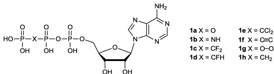
Fig. 6 Blackburn's ATP analogues [19].
