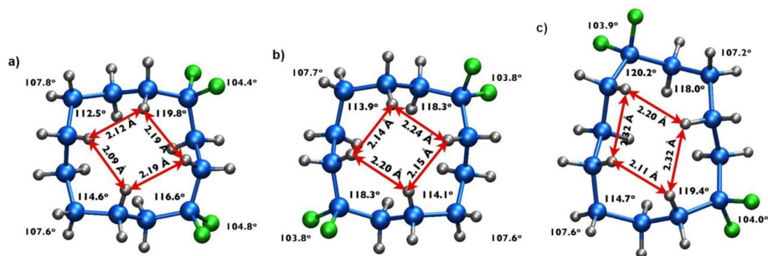
Fig. 13 (a) 1,1,4,4-, (b) 1,1,7,7-, and (c) 1,1,6,6-tetrafluorocyclododecanes [10]. The \text{CF}_2 groups occupy corner locations and will distort the ring to achieve this.
