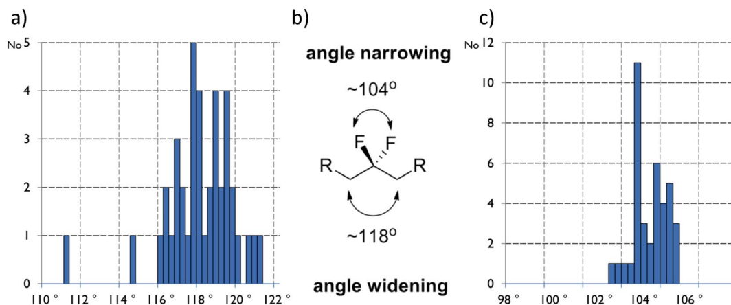
Fig. 1 Illustrates two histograms (a) and (c) which report a range of angles from 24 structures containing 39 ~CH 2 CF 2 CH 2 ~ motifs within the Cambridge Crystallographic Database. (a) C-CF 2 -C angles; (c) F-C-F angles; (b) is an illustrative summary of the average angles in this study [10].
