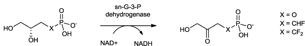
Fig. 8 Fluorophosphonate analogues of sn -glycerol-3-phosphate [22].
