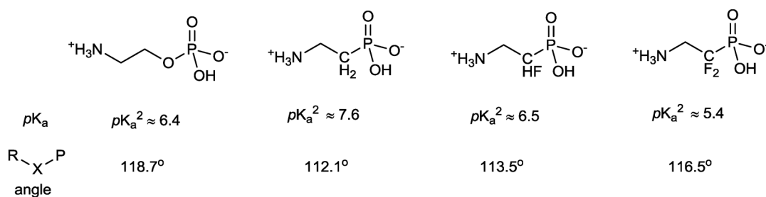
Fig. 7 Comparison of the C-X-P angles and pK_a^2 of phosphate and its phosphonate analogues.
