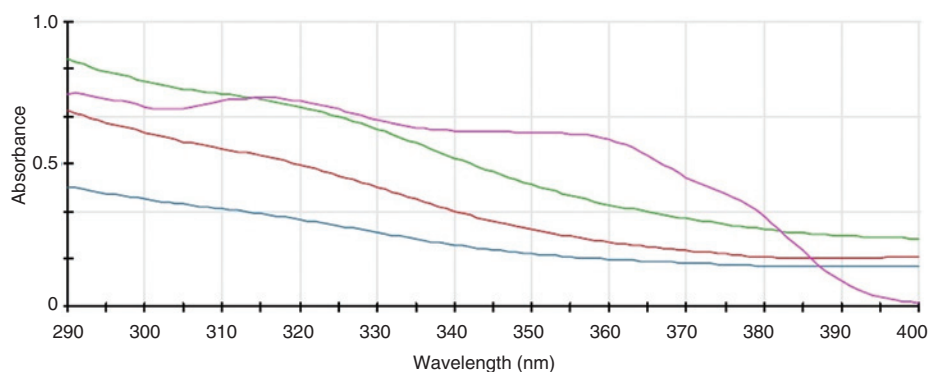
Fig. 2: UVA-UVB spectrum of S. meridense extracts and a mix of conventional sunscreens.
