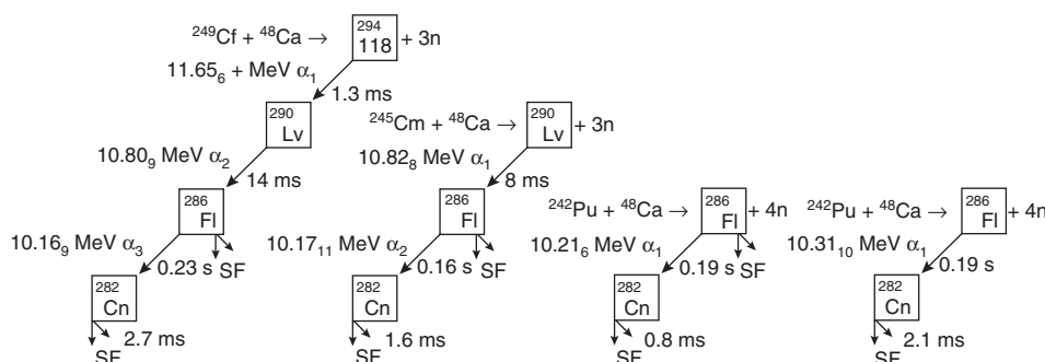
Fig. 2: Summary of the decay relevant work in the assignment of Z = 118 . The cross bombardments for the confirmation of identification of Z = 118 daughters provide firm evidence that a new atomic number, distinct from previously observed atomic numbers, has been identified. Alpha particle energies in MeV and lifetimes in milliseconds (ms) or seconds (s) are shown.
