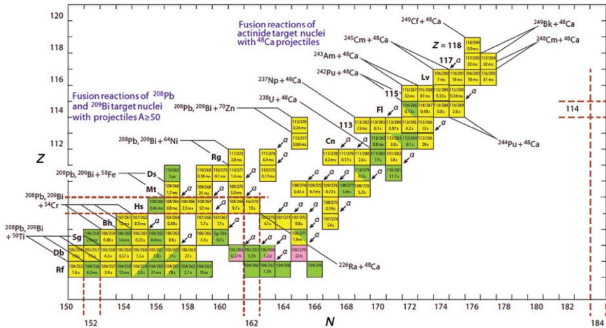
Fig. 1: Map of the region of superheavy nuclei relevant to this report including the reactions used to synthesize the various nuclides. (Adapted from [7].) The colors indicate different decay modes for nuclide Z/A along with its half life in milliseconds (ms), seconds (s), minutes (m) or hours (h) following the convention and data of [7], q, v .
