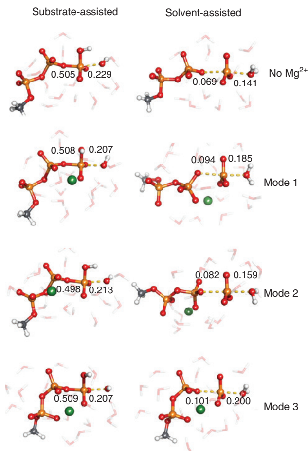
Fig. 4: Geometries of the lowest energy transition states for the substrate- and solvent-assisted hydrolyses of methyl triphosphate in aqueous solution, optimized using the \omega B97X-D functional, obtained as described in the Methodology section. The calculated bond orders to the incoming nucleophile and departing leaving group are also shown.
