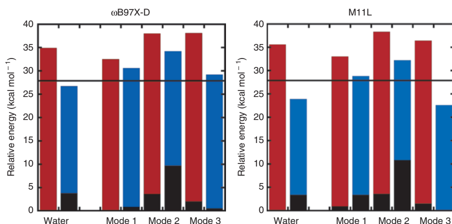
Fig. 3: A comparison of the calculated and experimental activation free energies ( \Delta G^\ddagger ) for methyl triphosphate hydrolysis, obtained using the (left) \omega B97X-D and (right) M11L functionals. The solid line indicates the experimental data ( \Delta G^\ddagger = 27.9 kcal·mol -1 ). Black bars: the variation in the ground-state energy relative to the lowest energy calculated ground state (see the Methodology section). The red bars show the transition state energy for the substrate-assisted pathway, the blue bars show the transition state energy for the solvent-assisted pathway.
