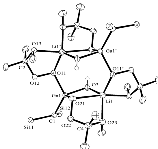
Fig. 2. Molecular structure of 5. The ellipsoids are drawn at the 40% probability level; hydrogen atoms with the exception of O-H are omitted. Selected bond lengths (pm) and angles (deg): Ga1–O11 189.1(1), Ga1–O21 190.5(1), Ga1–O3 186.0(1), Li1–O11' 194.0(3), Li1–O21 237.0(3), Li1–O13' 214.9(3), Li1–O23 204.3(3), Li1–O3 195.5(3), O11–O12 148.0(2), O21–O22 147.6(2); Ga1–O11–O12 103.42(8), Ga1–O21–O22 106.83(8), O11–O12–C2 108.3(1), O21–O22–C4 108.1(1), Ga1–O11–Li1' 121.1(1); Li1', O11' and O13' generated by -x+1, -y+1, -z+1 .
