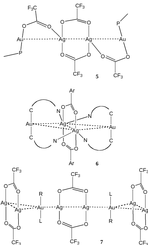
Scheme 3. Some complexes with Au...Ag metallophilic bonds.
