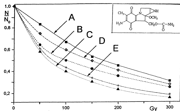
Fig. 2. Survival curves ( N/N_0 -ratio) of Escherichia coli (AB 1157) as a function of the absorbed dose (Gy) in aerated medium . (A) Buffer, (B) MMC, (C), MMC + vit. B1, (D) MMC + vit. B1 + vit. C, (E) MMC + vitamins: B1, C, E-ac. + \beta -car.; pH = 7.4, dose rate: 77 Gy/min; [MMC] = 1 \times 10^{-6} M; [vit. B1] = [vit. C] = [E-ac] = [ \beta -car] = 1 \times 10^{-4} M.
