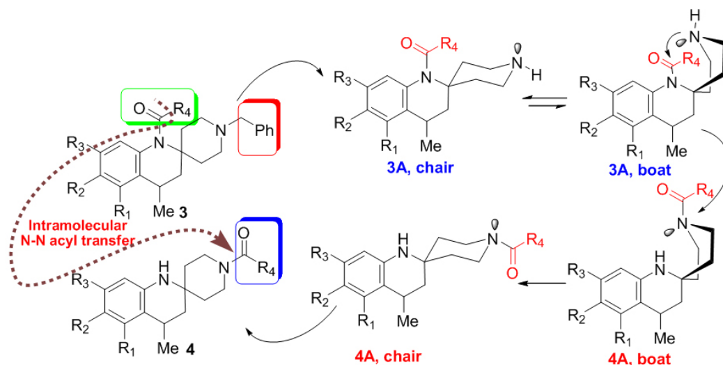
Scheme 7. Intramolecular acyl transfer reaction in spiro piperidine system 4 .
