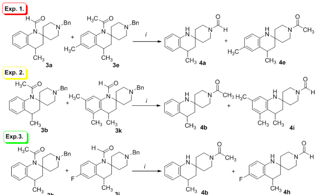
Scheme 4. Possible products of debenzylation process.
