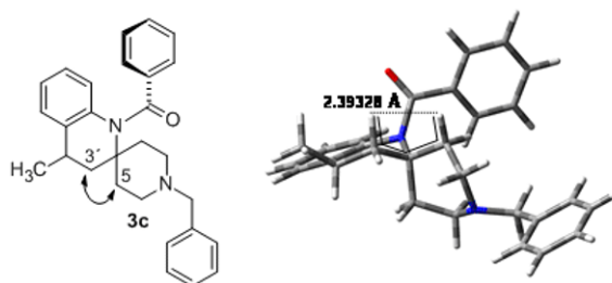
Figure 3. Capped-stick model of lowest energy of compound 3c .
