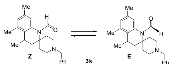
Figure 2. Z - and E -isomers of formamide 3k .
