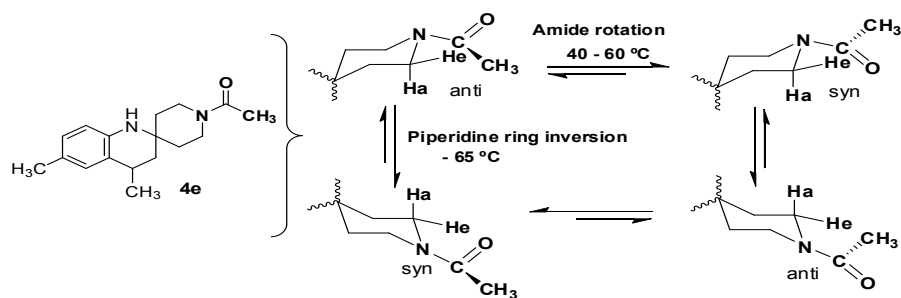
Scheme 3. Conformational equilibrium for acetamide 4e .
