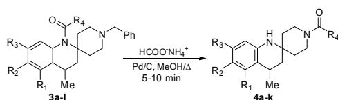
Scheme 2. Preparation of new 1-acyl-3',4'-dihydro-1'H-spiro[piperidine-4,2'-quinolines] 4 .
