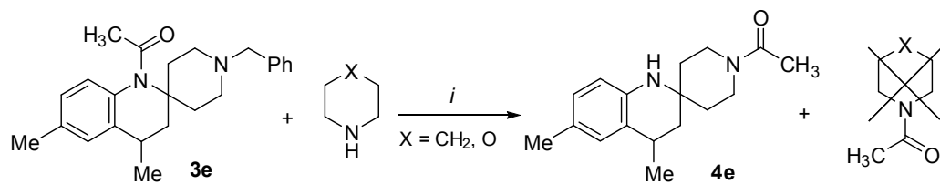
Scheme 5. Crossover experiments of two different amides.
