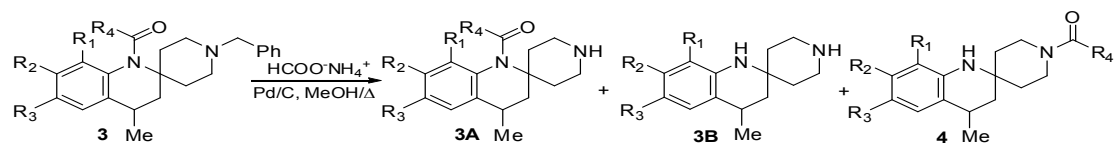
Scheme 4. Possible products of debenzylation process.
